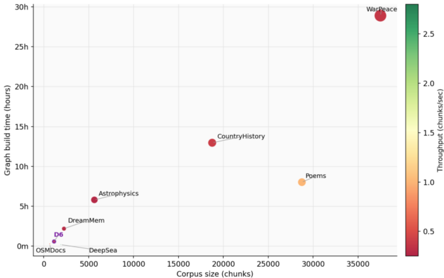
Build Time vs Corpus Size (bubble size = entity count, colour = throughput)
