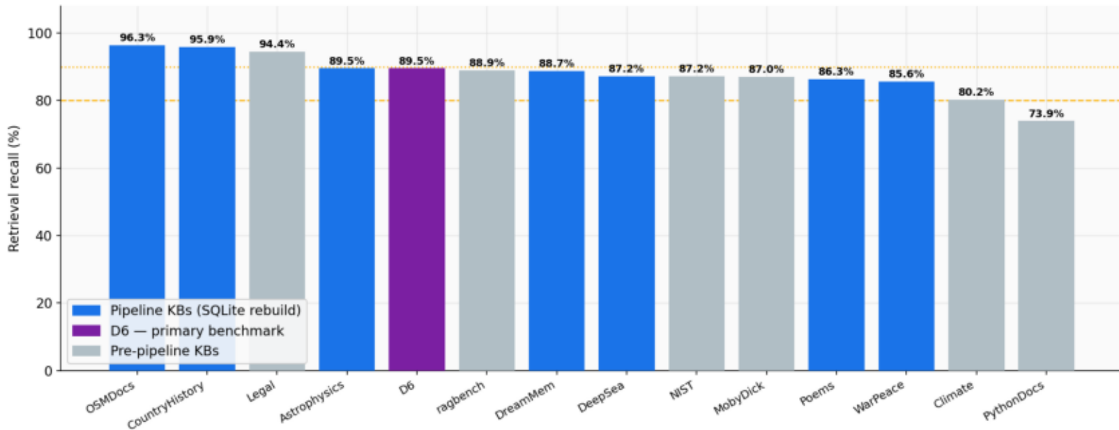
Retrieval Recall — All 14 Knowledge Bases (Ranked)
