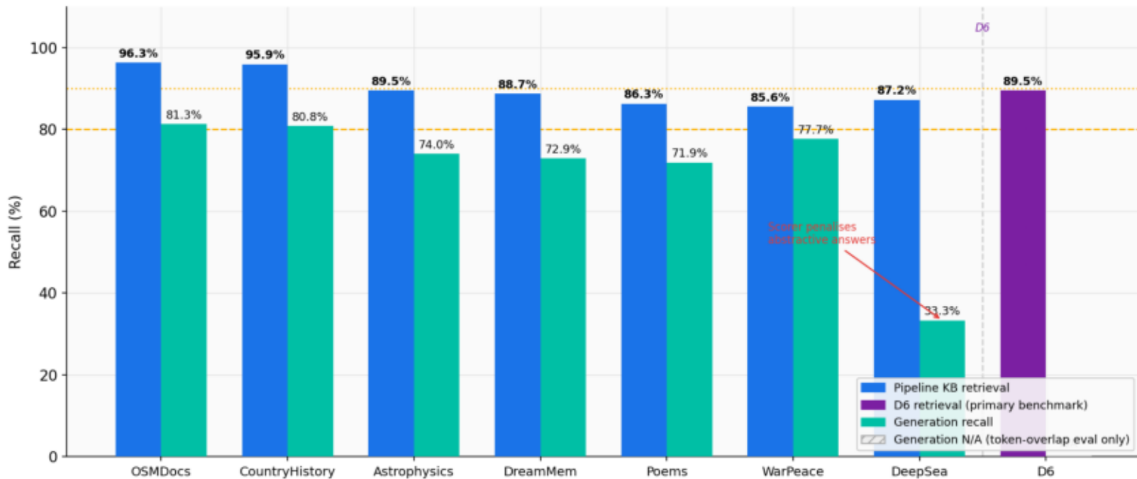
Retrieval & Generation Recall — Pipeline KBs + D6 Primary Benchmark
