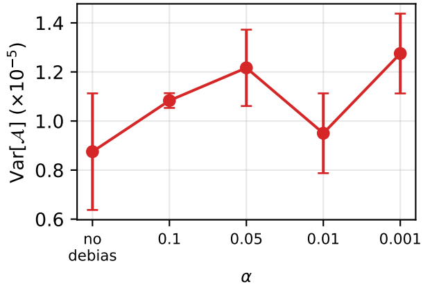
Variance across groups
