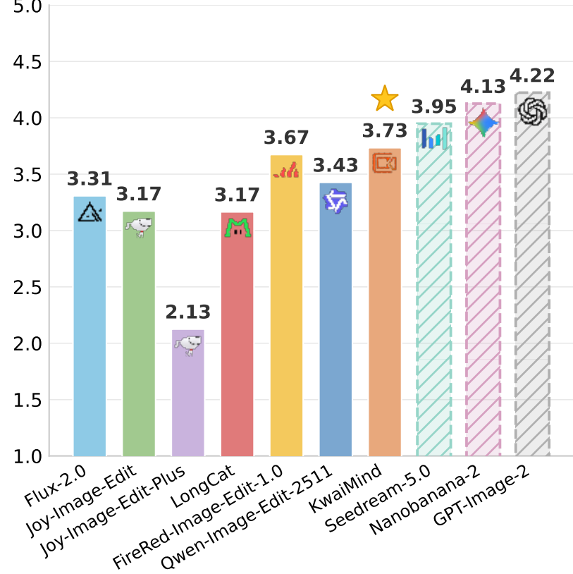
REDEdit (CN)
