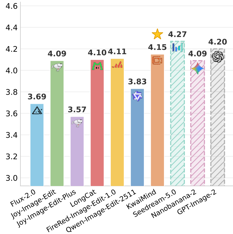
ImgEdit (Gemini)
