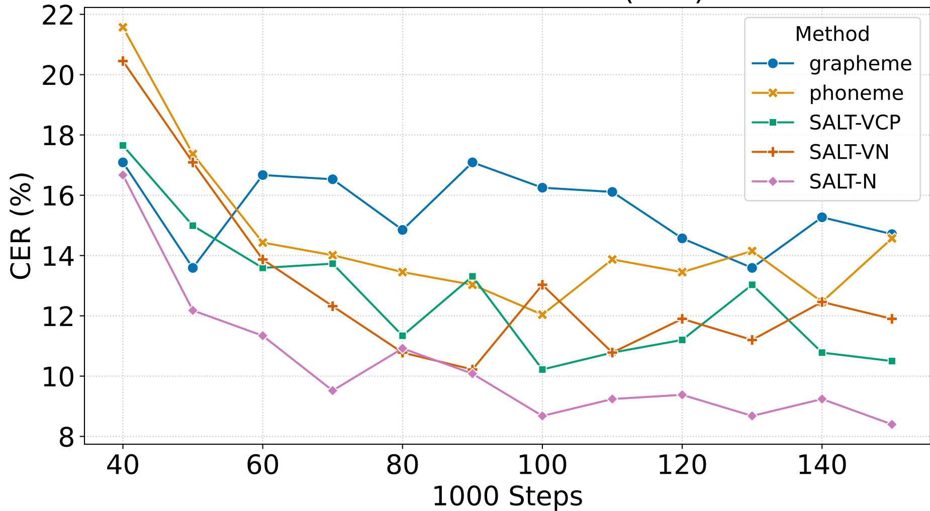
Character Error Rate (CER)
