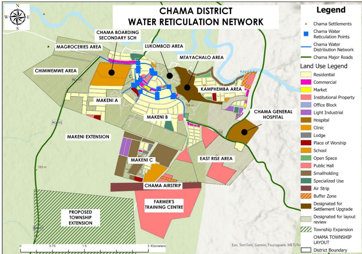
Figure 6: Layout of the Urban Water Reticulation Network
