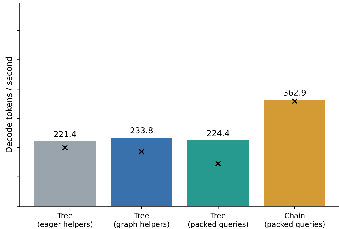
LayerSkip-Llama3-8B + Qwama-0.5B
