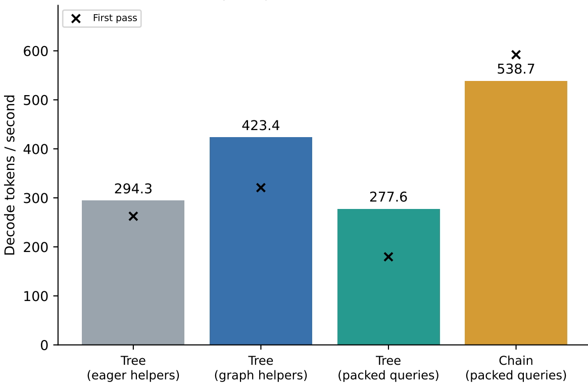
LayerSkip-Llama2-7B + AMD-135M
