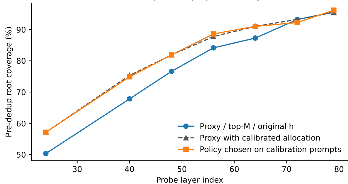
Held-out snapshot replay, root budget 15
