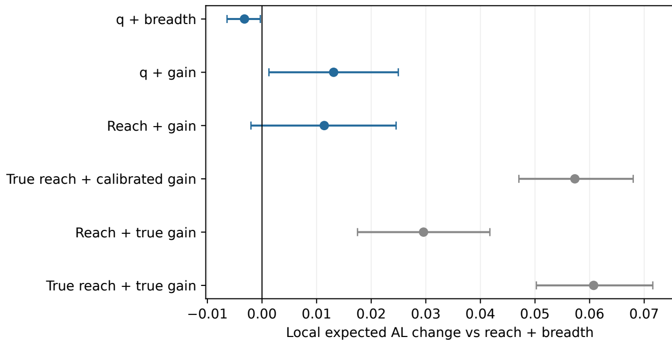
C=3 allocation diagnostic — observed parent pool; not online AL
