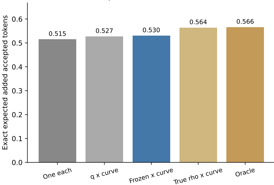
Same two-parent / two-new-node decision
