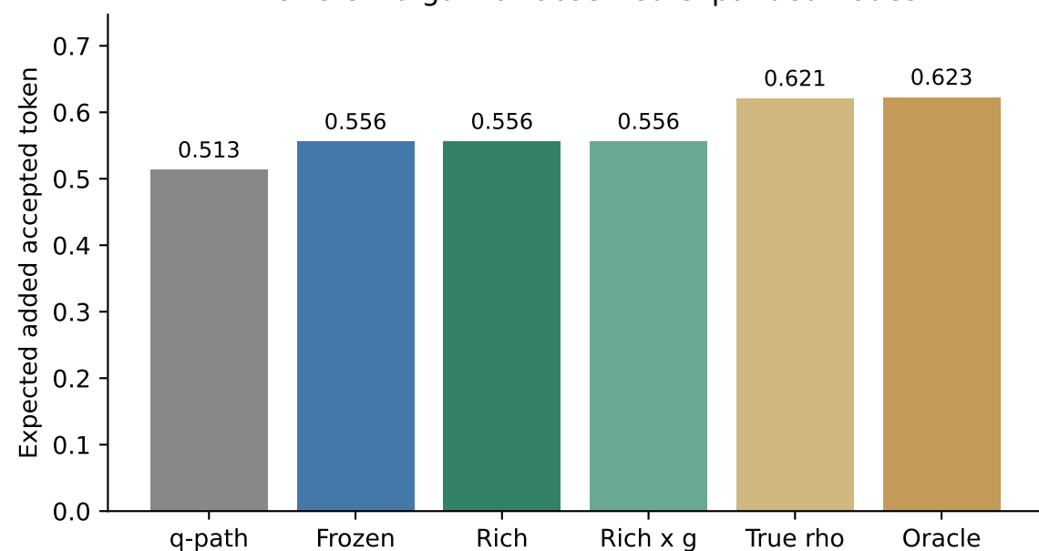
D One-child gain at observed expanded nodes
