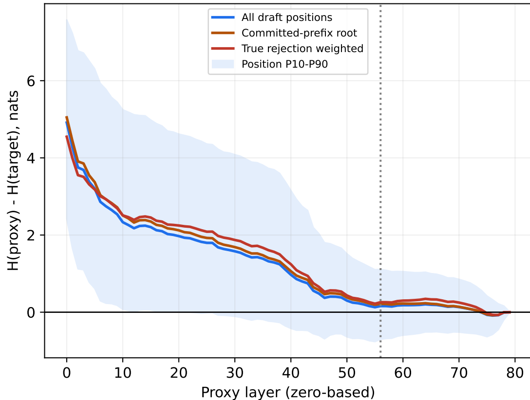
Entropy difference across proxy layers
