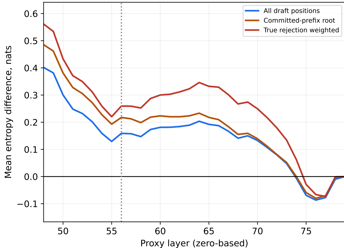
Late layers: mean difference can change sign
