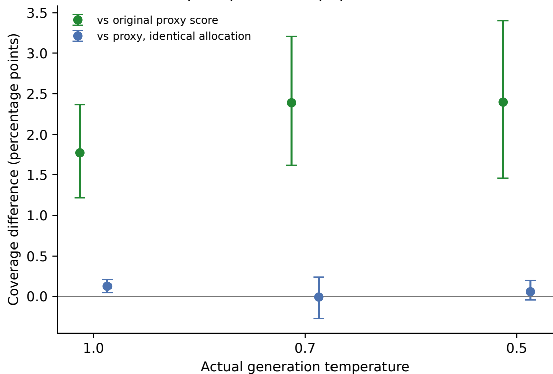
Paired prompt bootstrap, pointwise 95% CI
