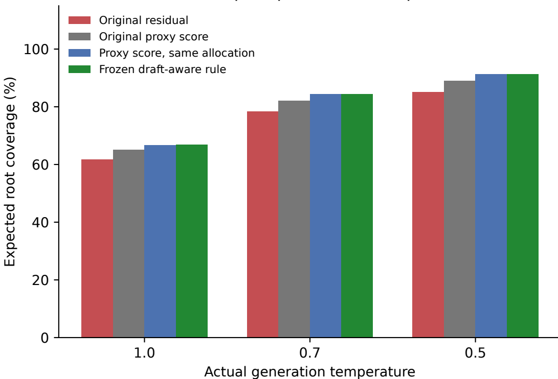
96 unseen prompts at each temperature
