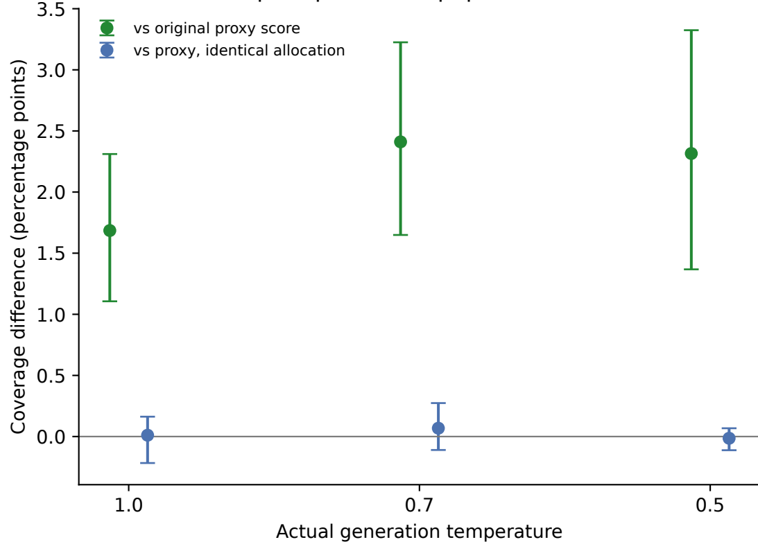
Paired prompt bootstrap, pointwise 95% CI
