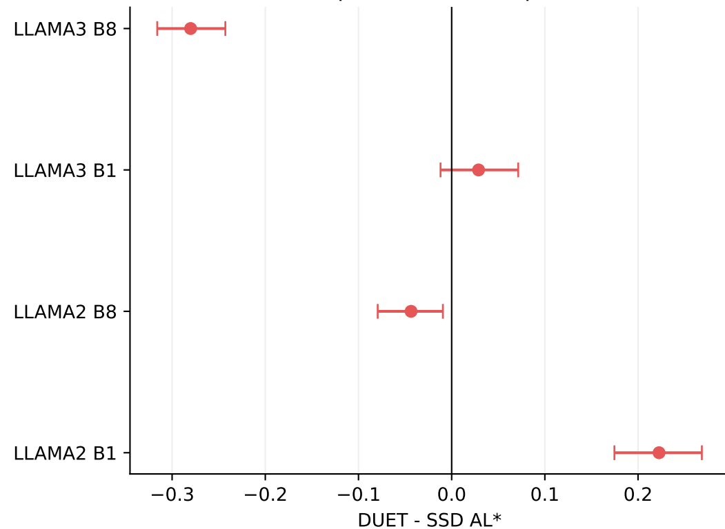
Full480, question bootstrap 95% CI
