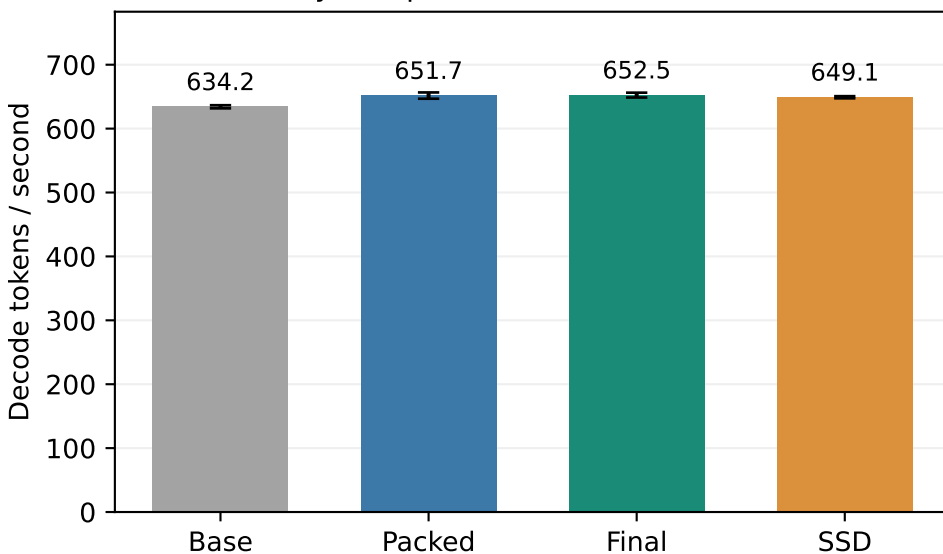
LayerSkip-Llama2-7B + AMD135M
