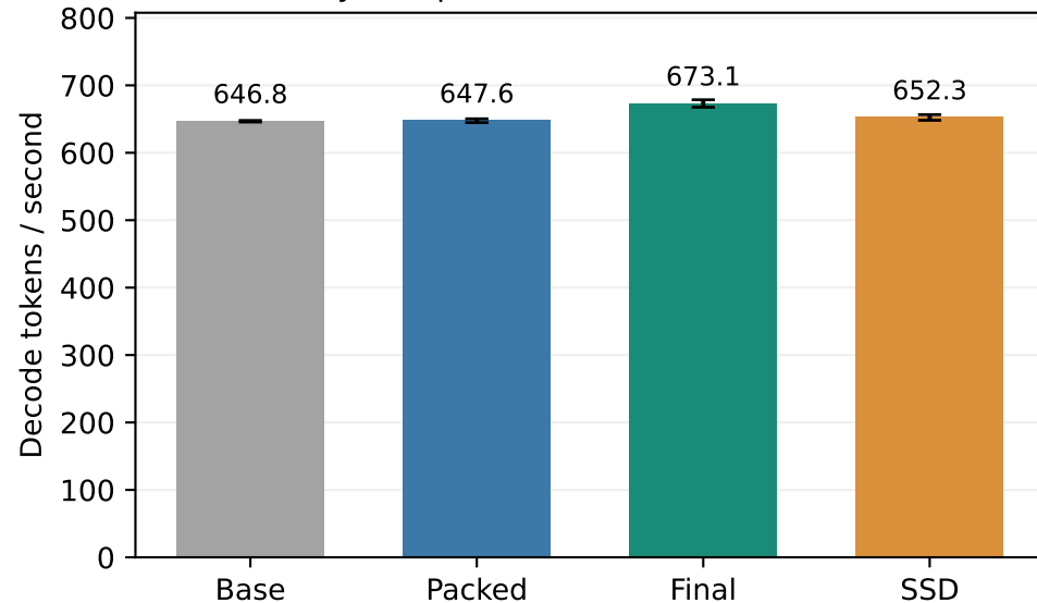
LayerSkip-Llama3-8B + Qwama0.5B
