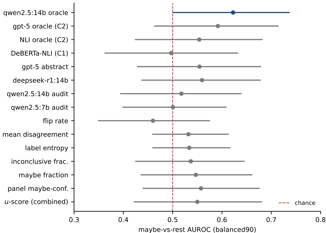
Uncertainty signals vs. chance (95% bootstrap CI)
