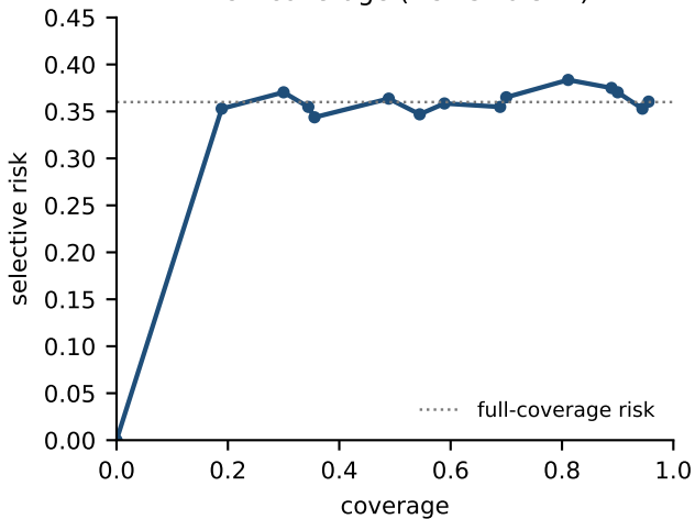
Risk-coverage (AURC=0.311)
