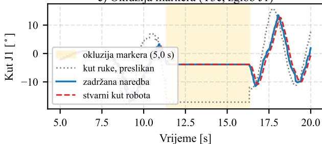
c) Okluzija markera (T3c, zglob J1)
