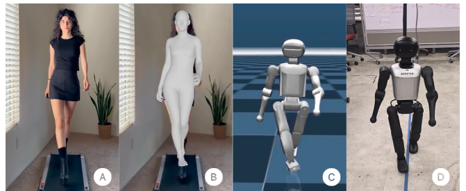
Fig. 1. Overview of the pipeline: (a) monocular runway video, (b) recovered 3D human motion, (c) retargeted robot motion in simulation, and (d) physical deployment on the Booster K1.
