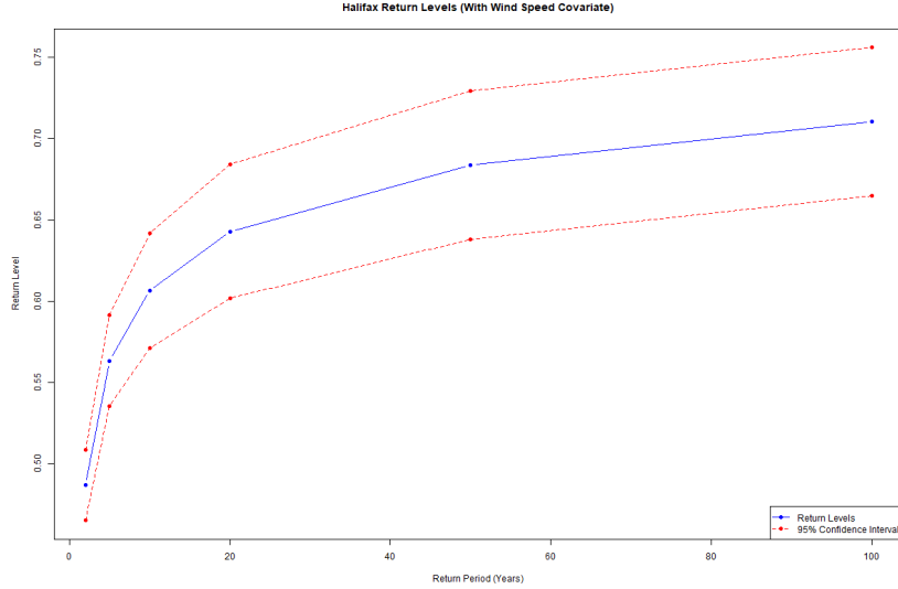
Figure 18: Halifax Return Level Plot - Covariate Case
