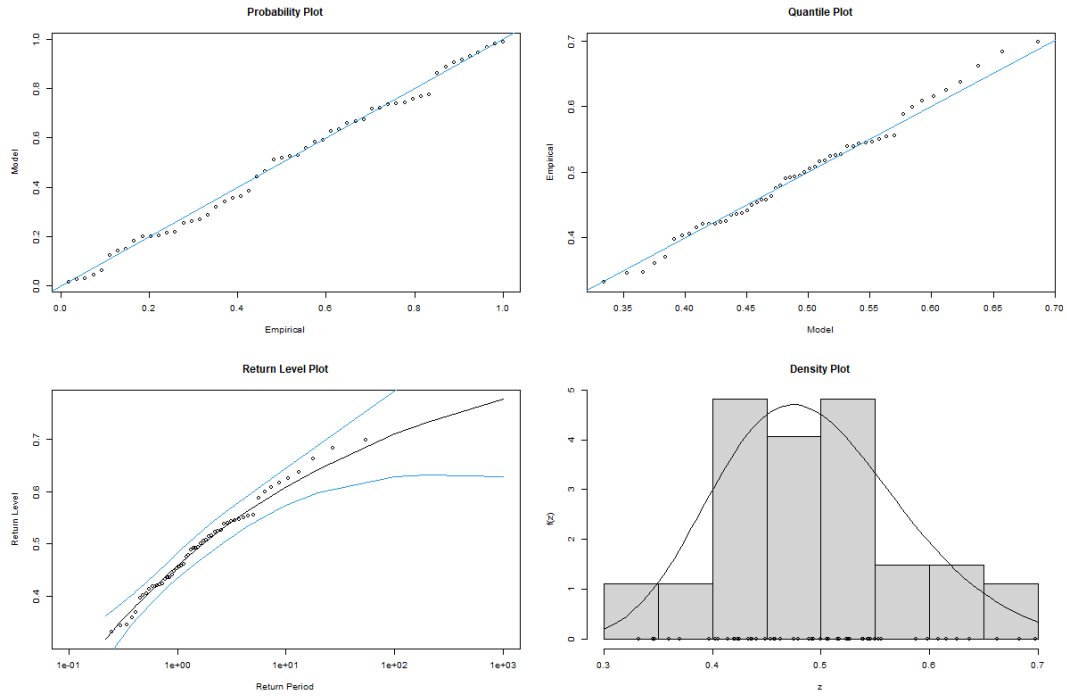
Figure 23: Yarmouth Diagnostics plots from the GEV fit - Non Covariate Case
