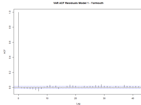
Figure 19: ACF plot of residuals of VAR(7) model for Yarmouth.
