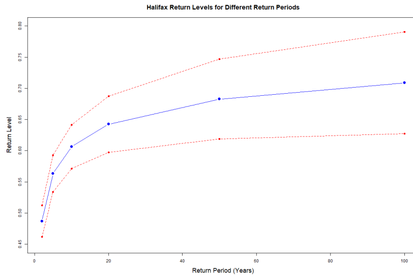
Figure 24: Halifax Return Level Plot - Non Covariate Case
