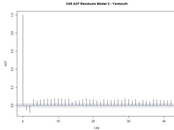
Figure 17: ACF plot of residuals of VAR(1) model of water surge and wind speed in Yarmouth.
