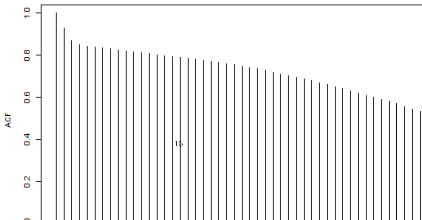
Halifax-ACF-Temperature
