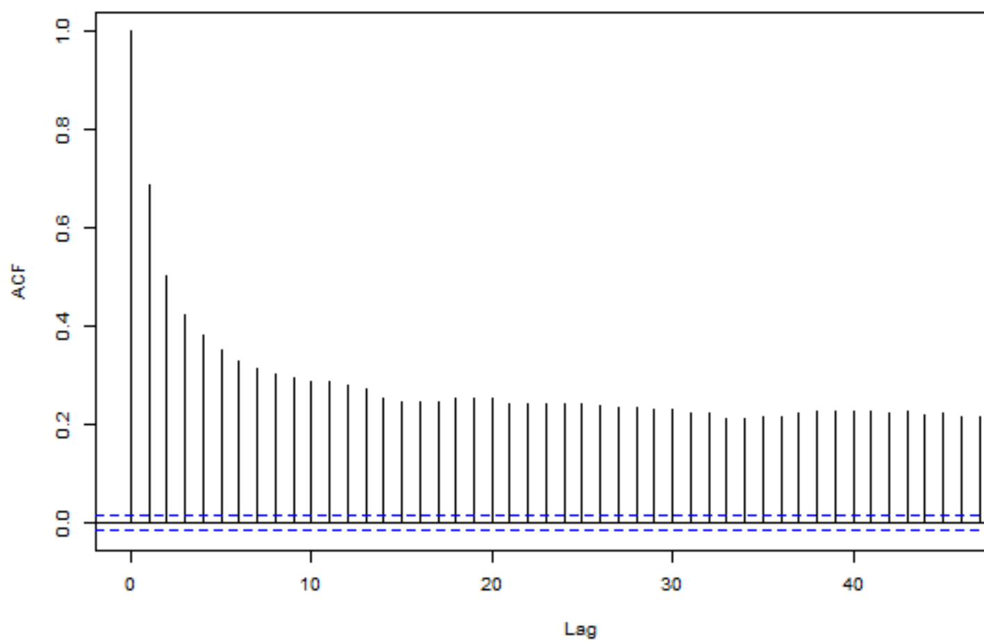
Halifax-ACF-Temperature
