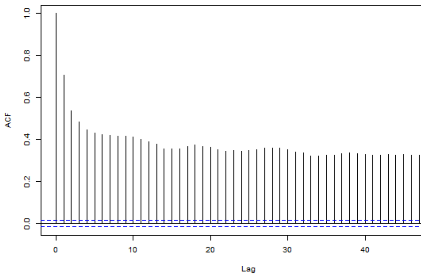
Yarmouth-ACF-Temperature
