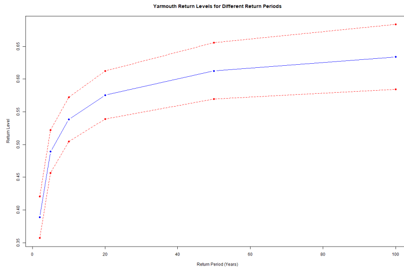
Figure 24: Yarmouth Return Level Plot - Non Covariate Case
