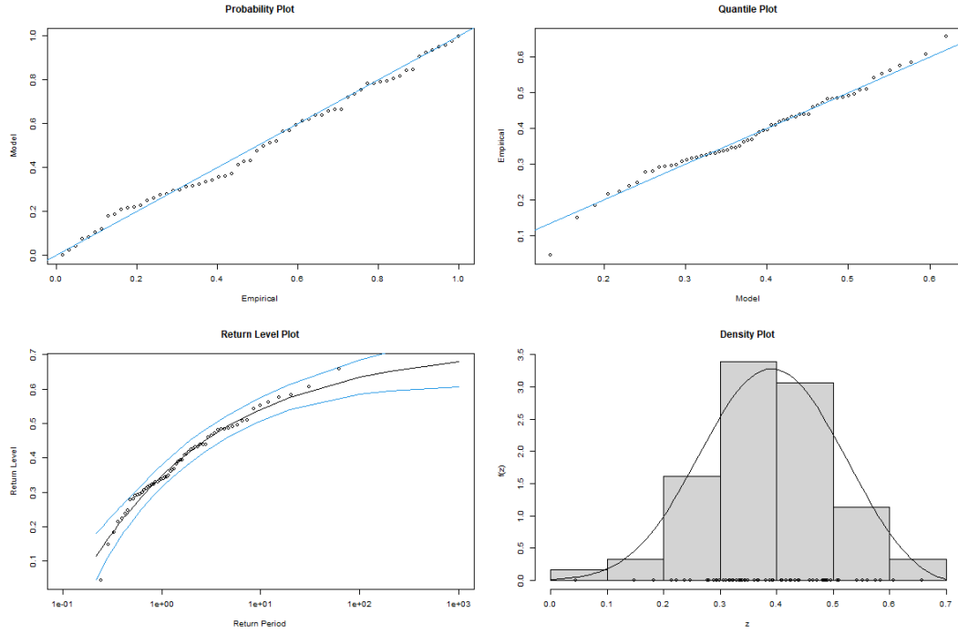
Figure 23: Yarmouth Diagnostics plots from the GEV fit - Non Covariate Case
