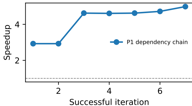
Stencil3d B
