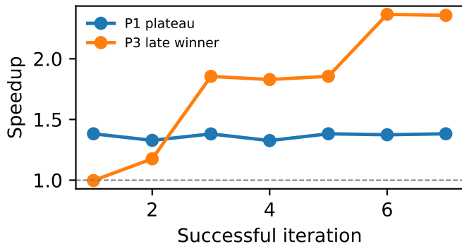
Bitonic A
