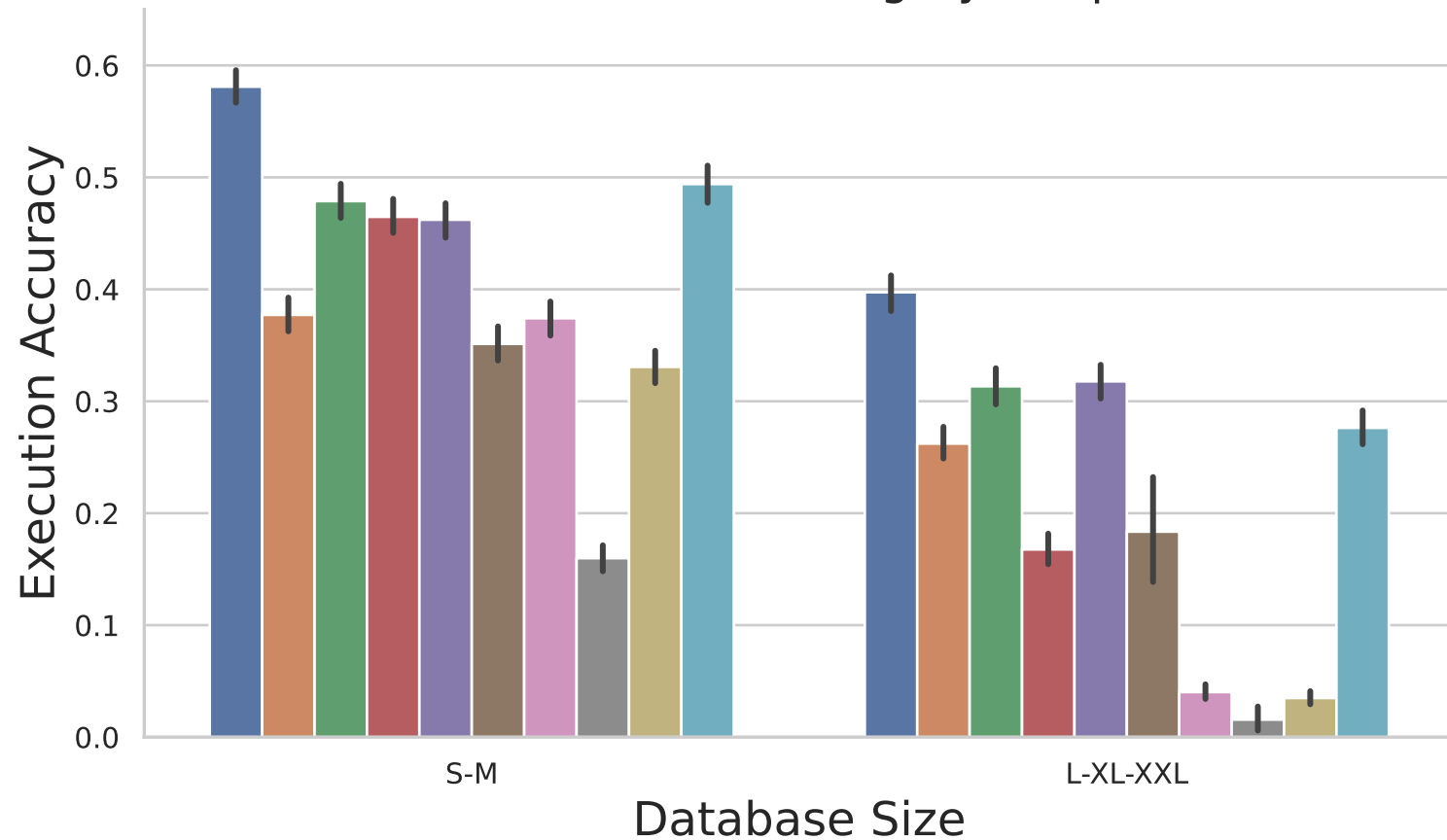
NL to SQL LLM Category = Open
