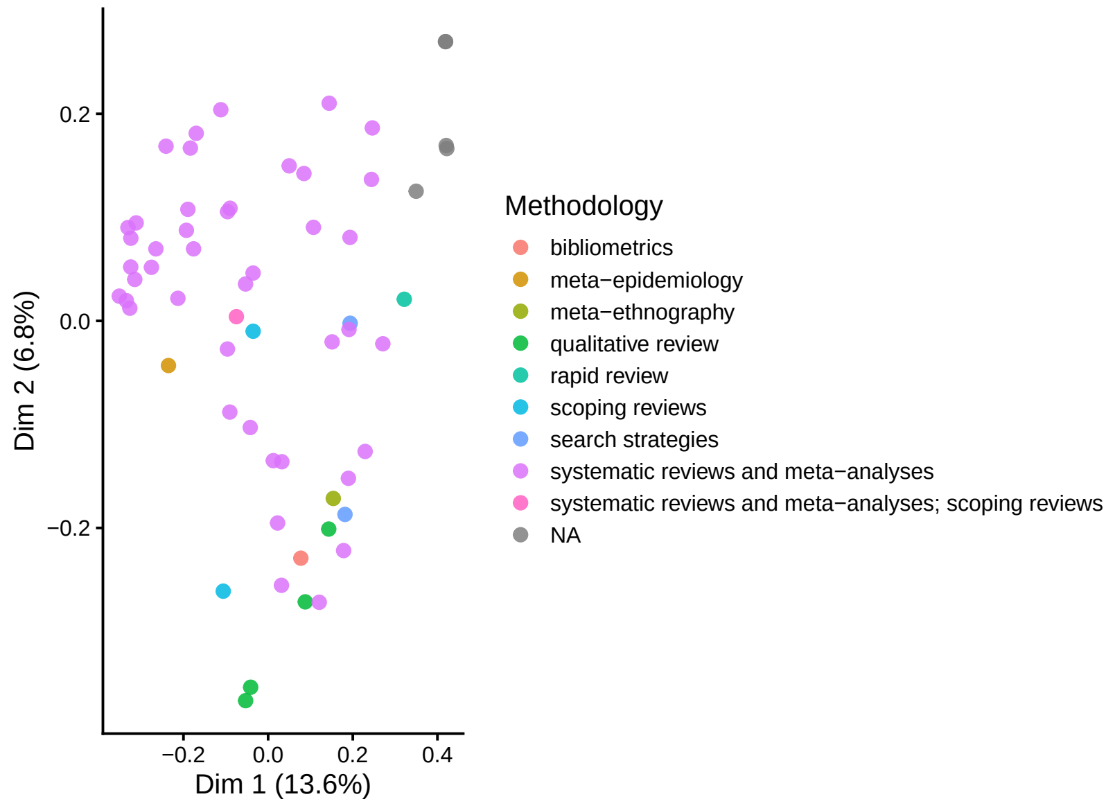
MDS of checklists by concept overlap (Jaccard distance)
