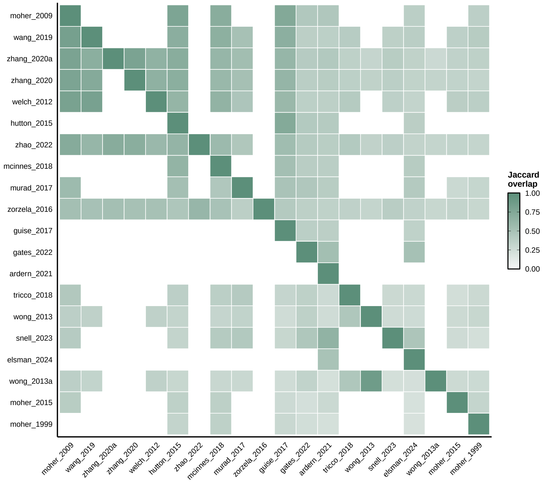
Top 20 guidelines by mean pairwise concept overlap
