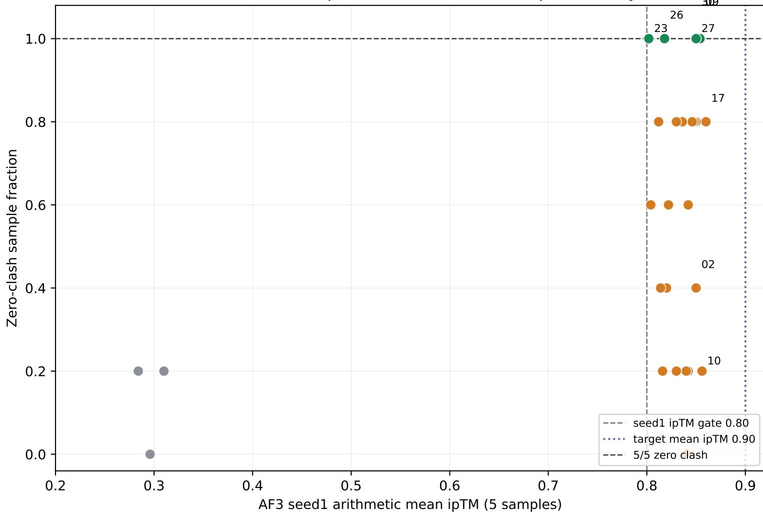
E252 AF3 seed1: ipTM vs 2.4 A zero-clash reproducibility
