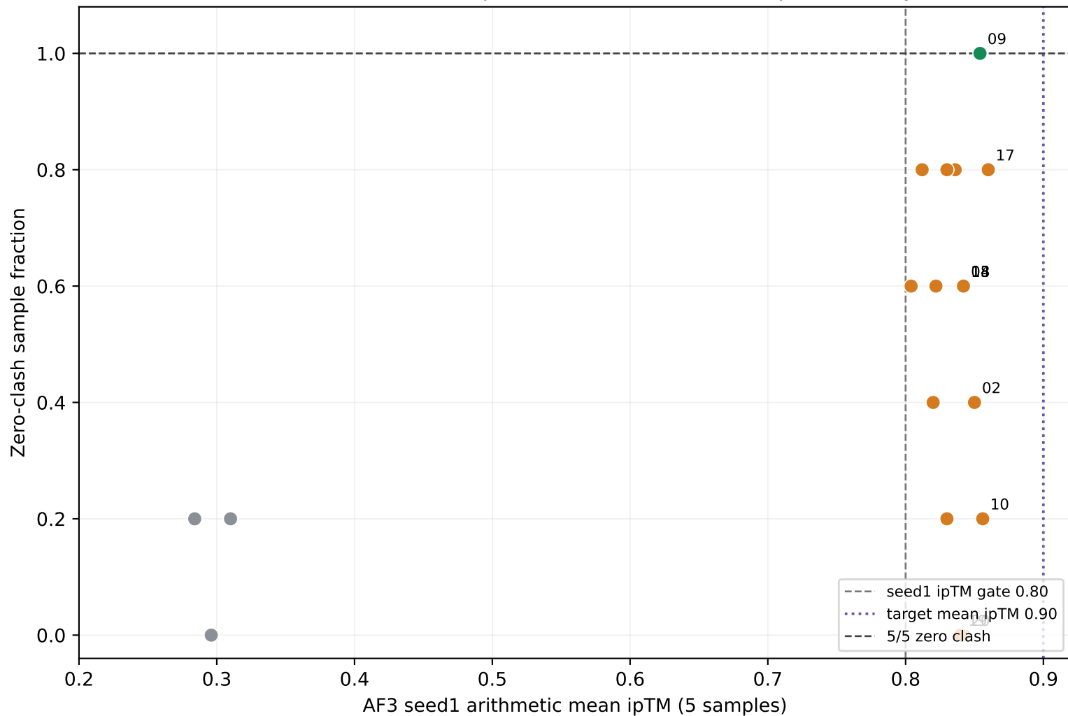
E252 AF3 seed1 live: ipTM vs 2.4 A zero-clash reproducibility
