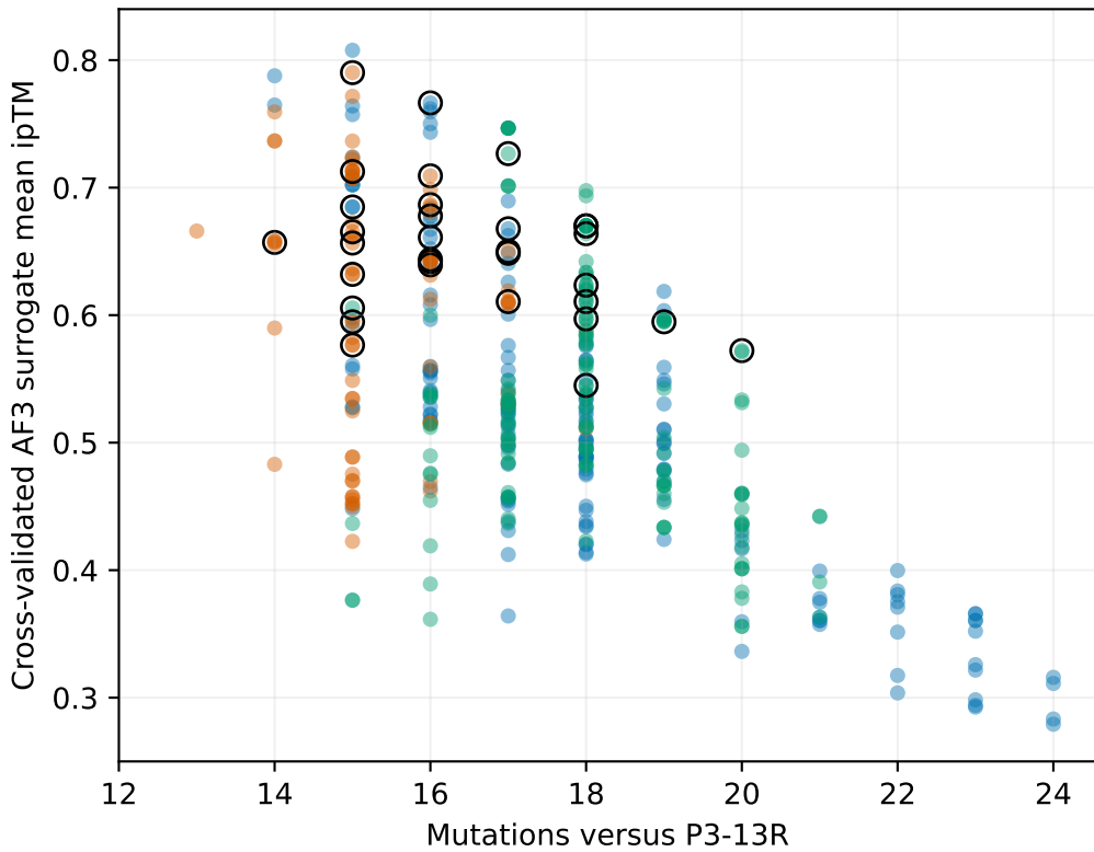
Mutation budget and E257 selection
