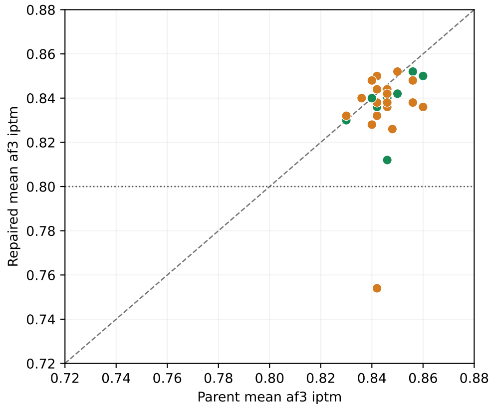
AF3 clash-directed repair effect (32 completed candidates)
