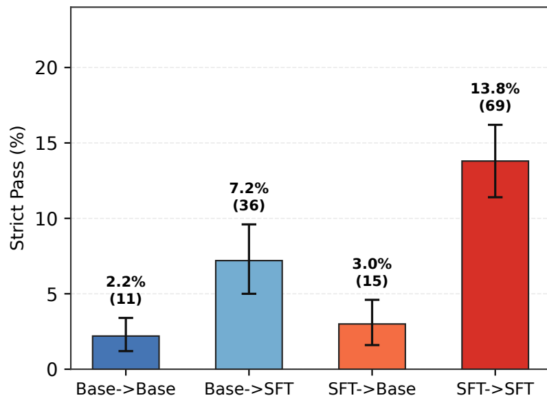
Phi-4: Strict Rate (%)
