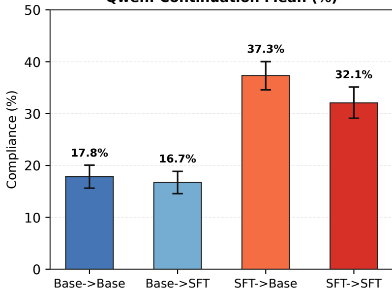
Qwen: Continuation Mean (%)
