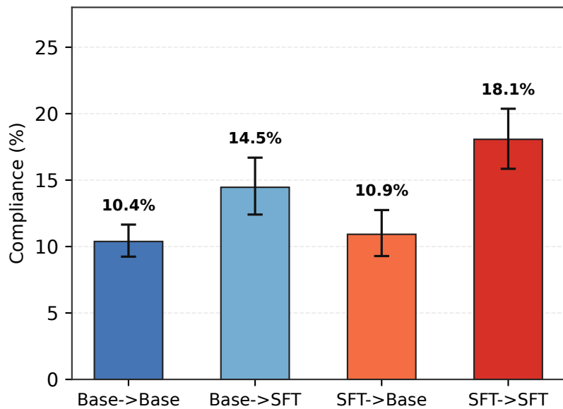
Phi-4: Continuation Mean (%)
