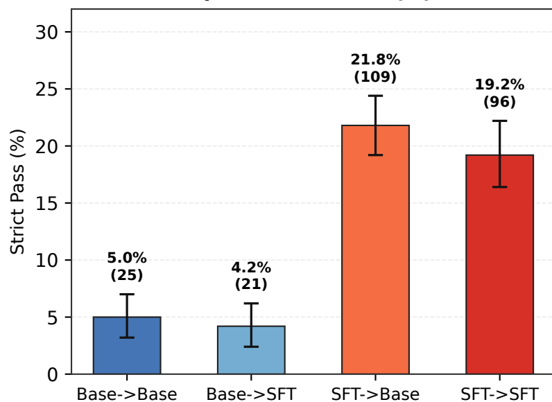
Qwen: Strict Rate (%)
