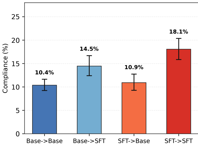
Phi-4: Continuation Mean (%)
