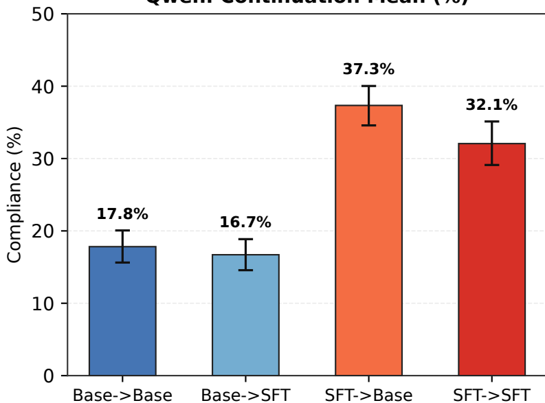
Qwen: Continuation Mean (%)
