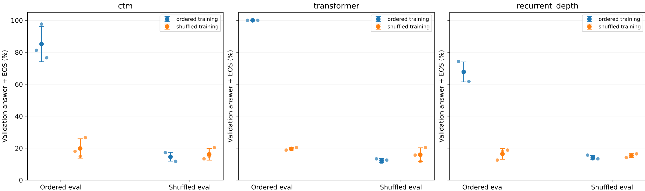
Fixed update3000: paired development seeds23/29/31, mean \pm sample SD
