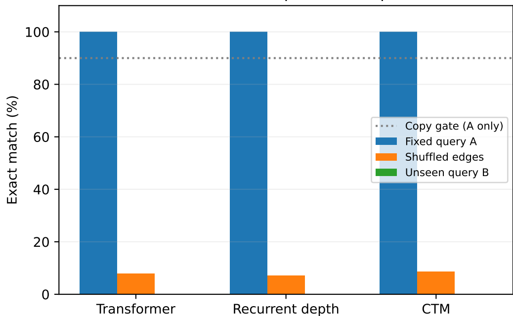
Same held-out maps: transfer probes
