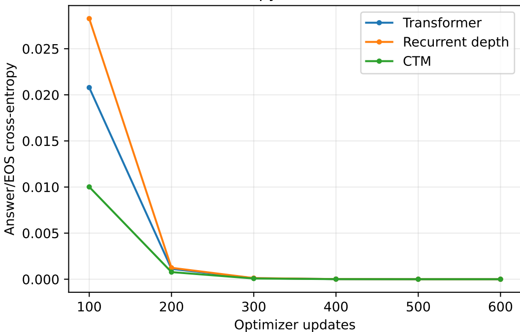
Fixed-copy validation loss
