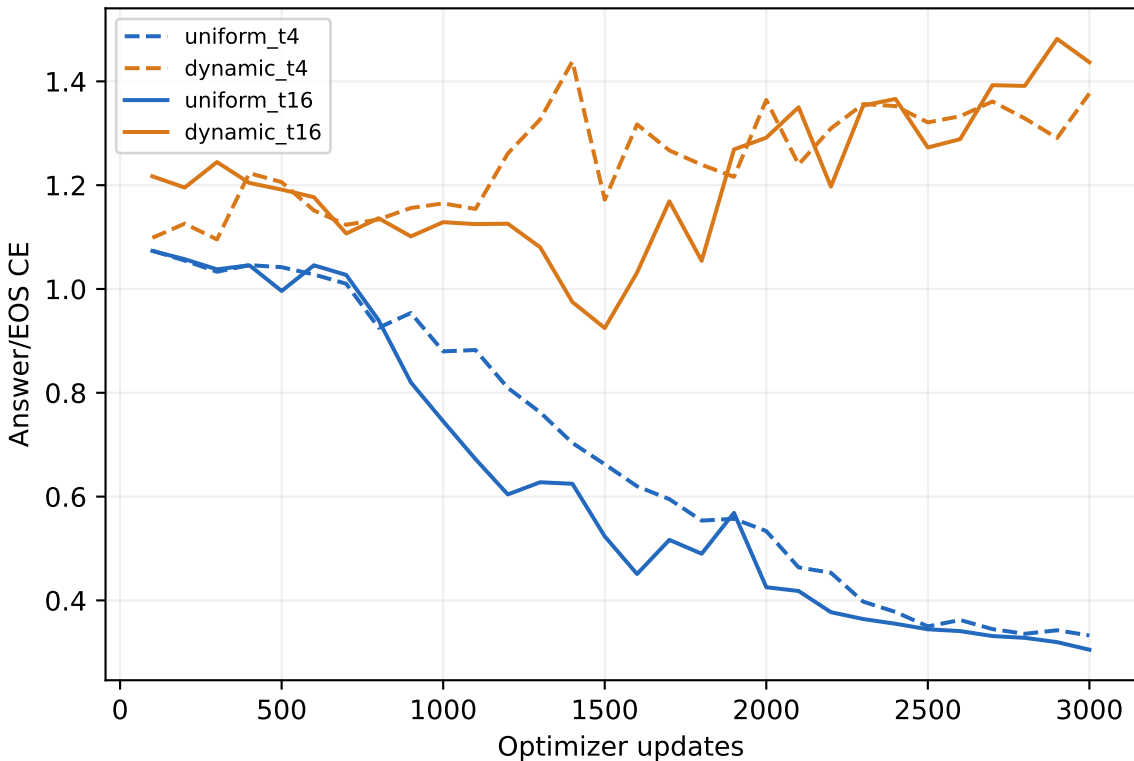
Common final-trained-tick validation CE
