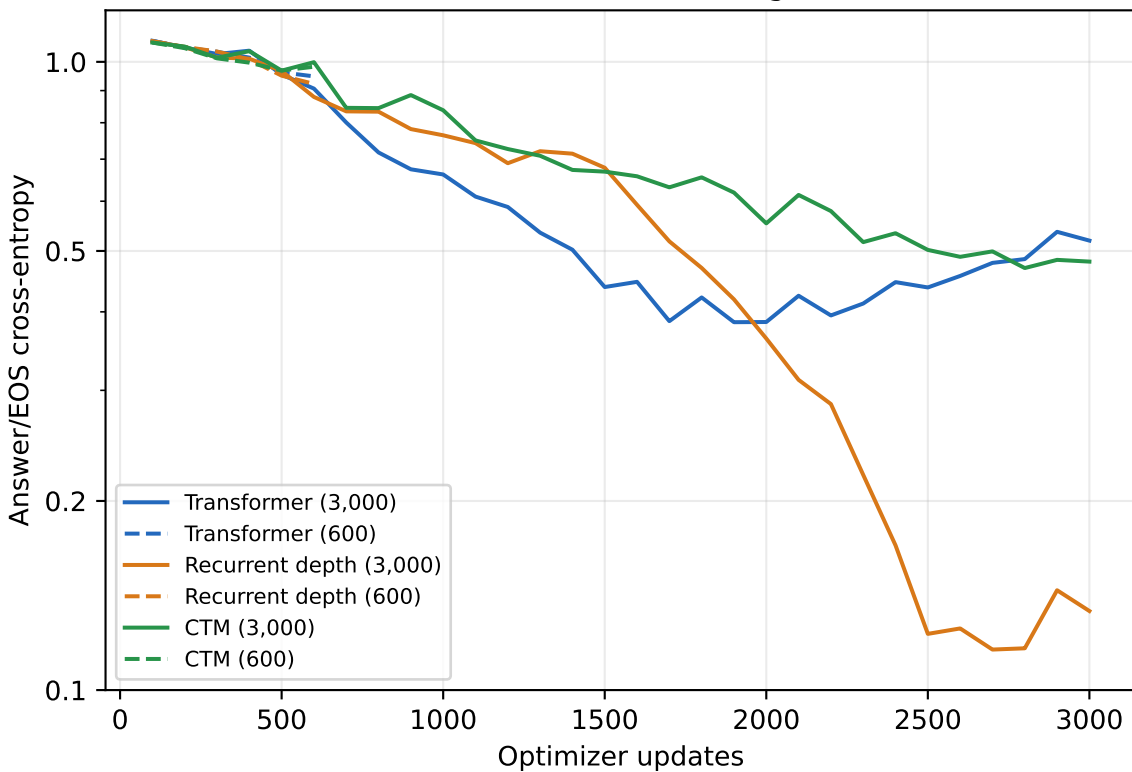
Validation loss: distinct training schedules
