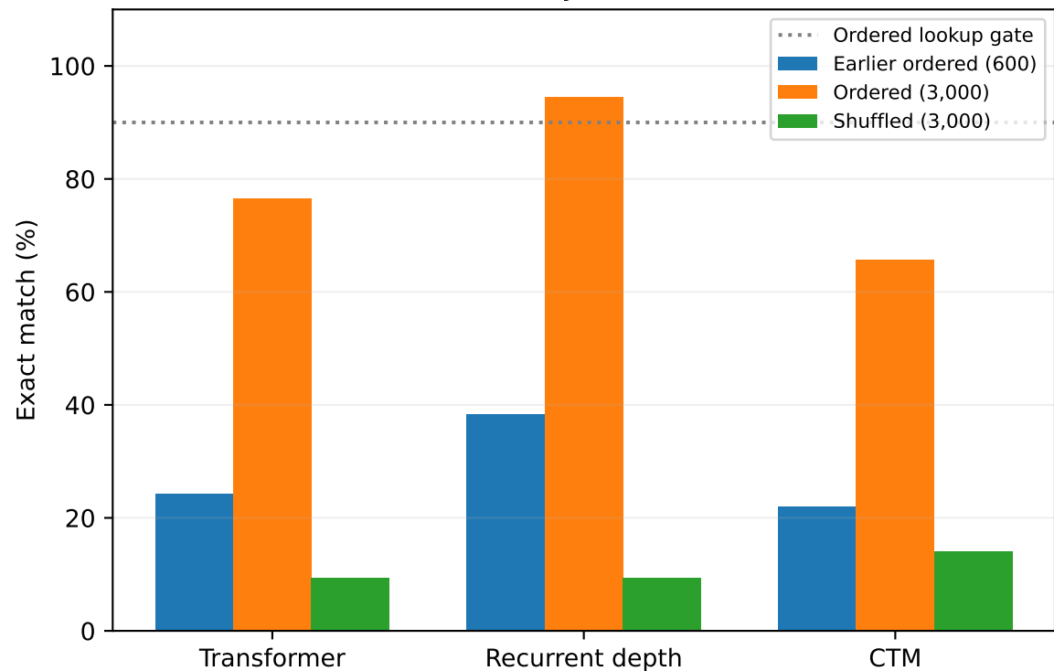
Held-out accuracy and order transfer
