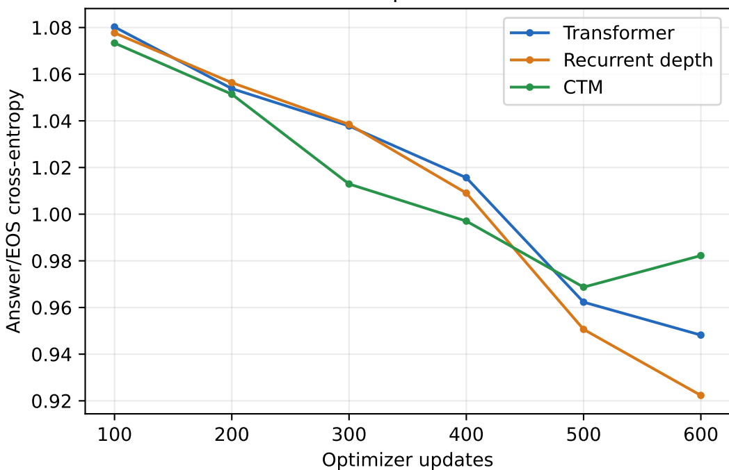
Ordered lookup: validation loss
