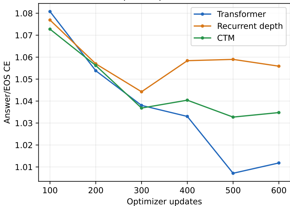
One-hop lookup: validation loss
