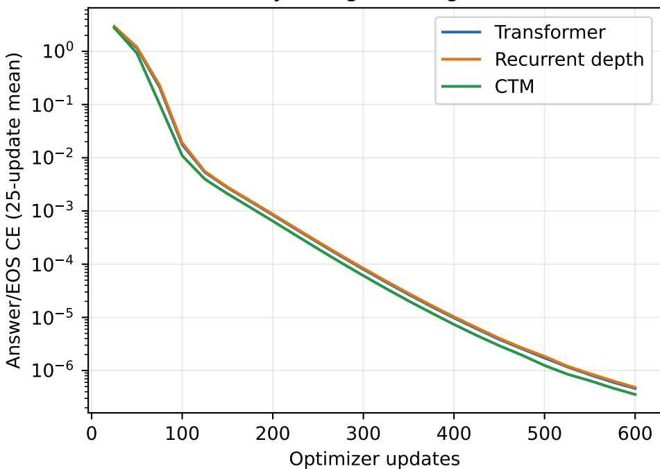
Tiny fitting: training loss
