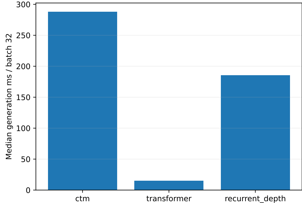
Frozen winners: test quality and measured generation cost on RTX 3090
