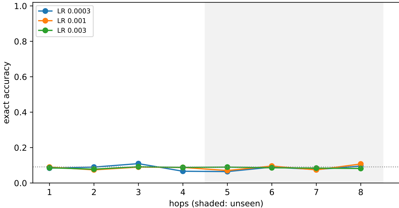
Multi-hop training, final checkpoint
