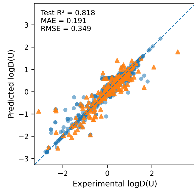
ExtraTrees
