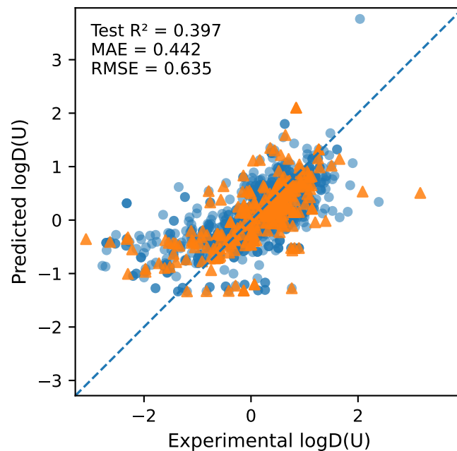
RandomForest
