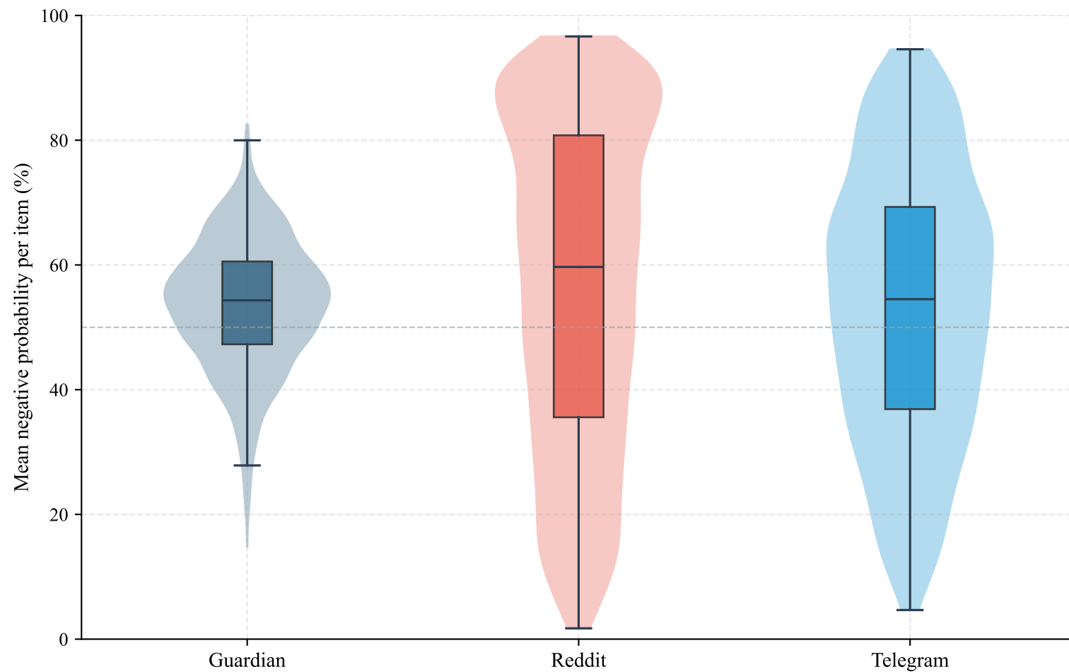
(a) Item-level negativity distribution
