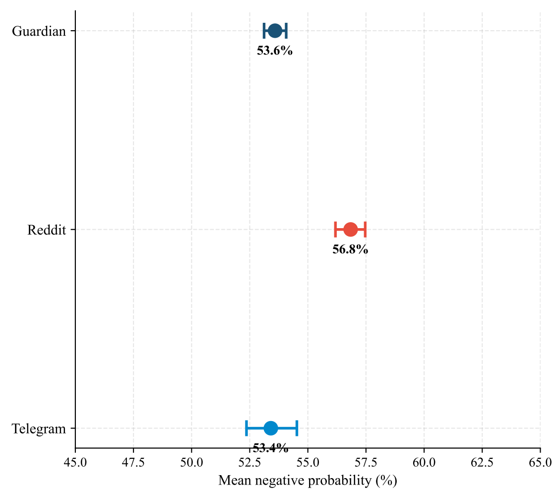
(b) Platform mean \pm 95% CI
