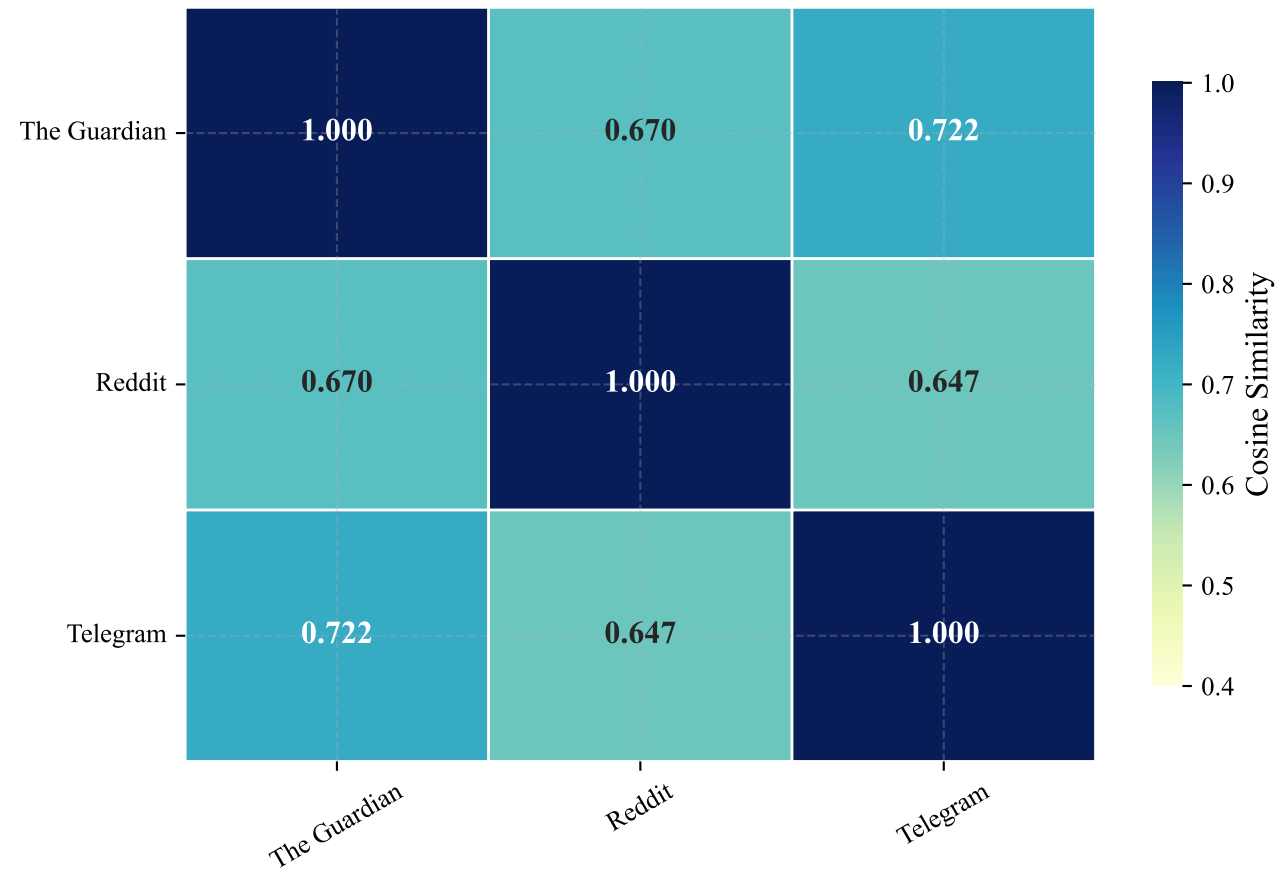
(a) Cosine Similarity
