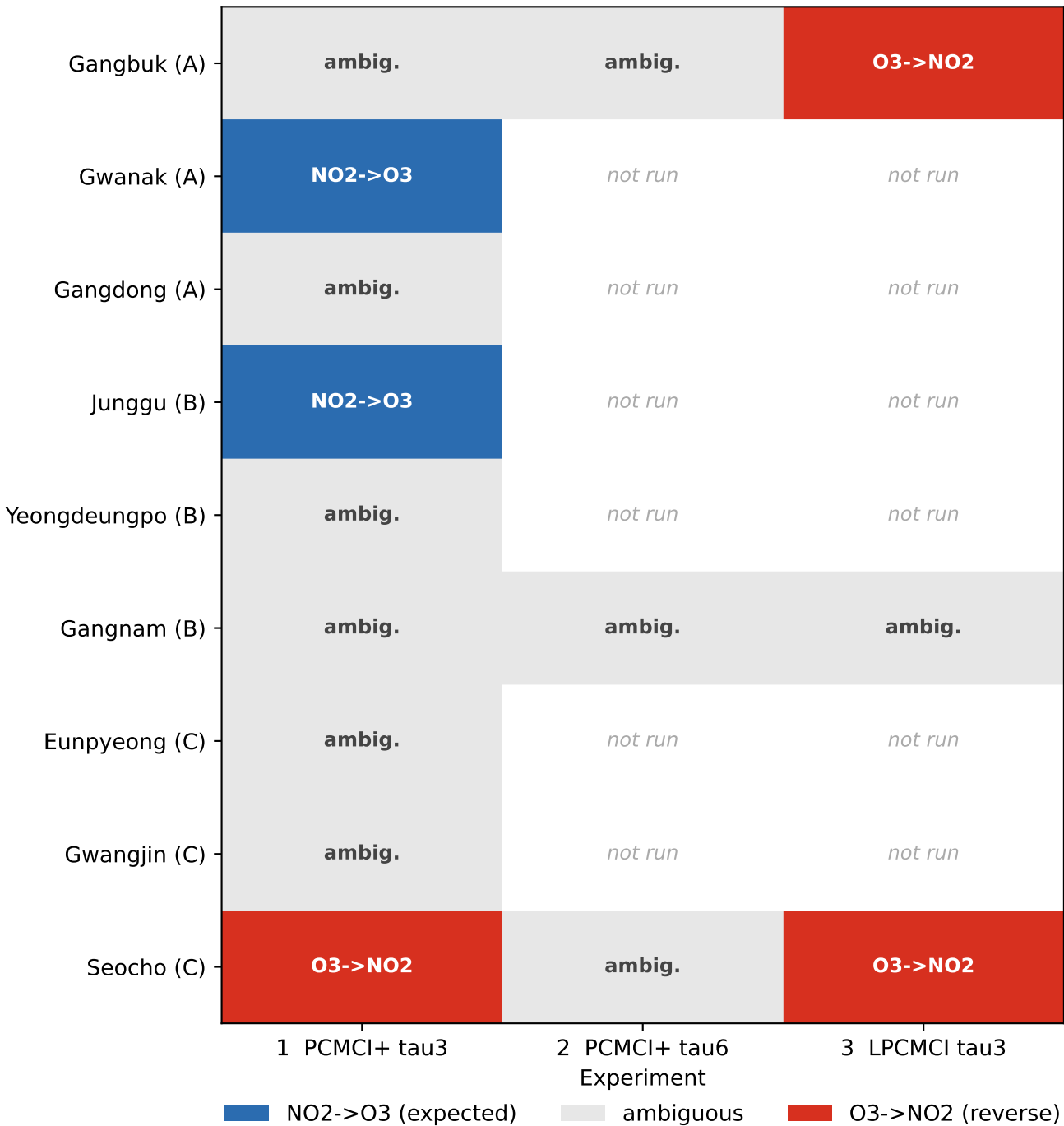
NO2-O3 contemporaneous direction across stations and audit settings Blue: expected direction; red: reverse; gray: unresolved
