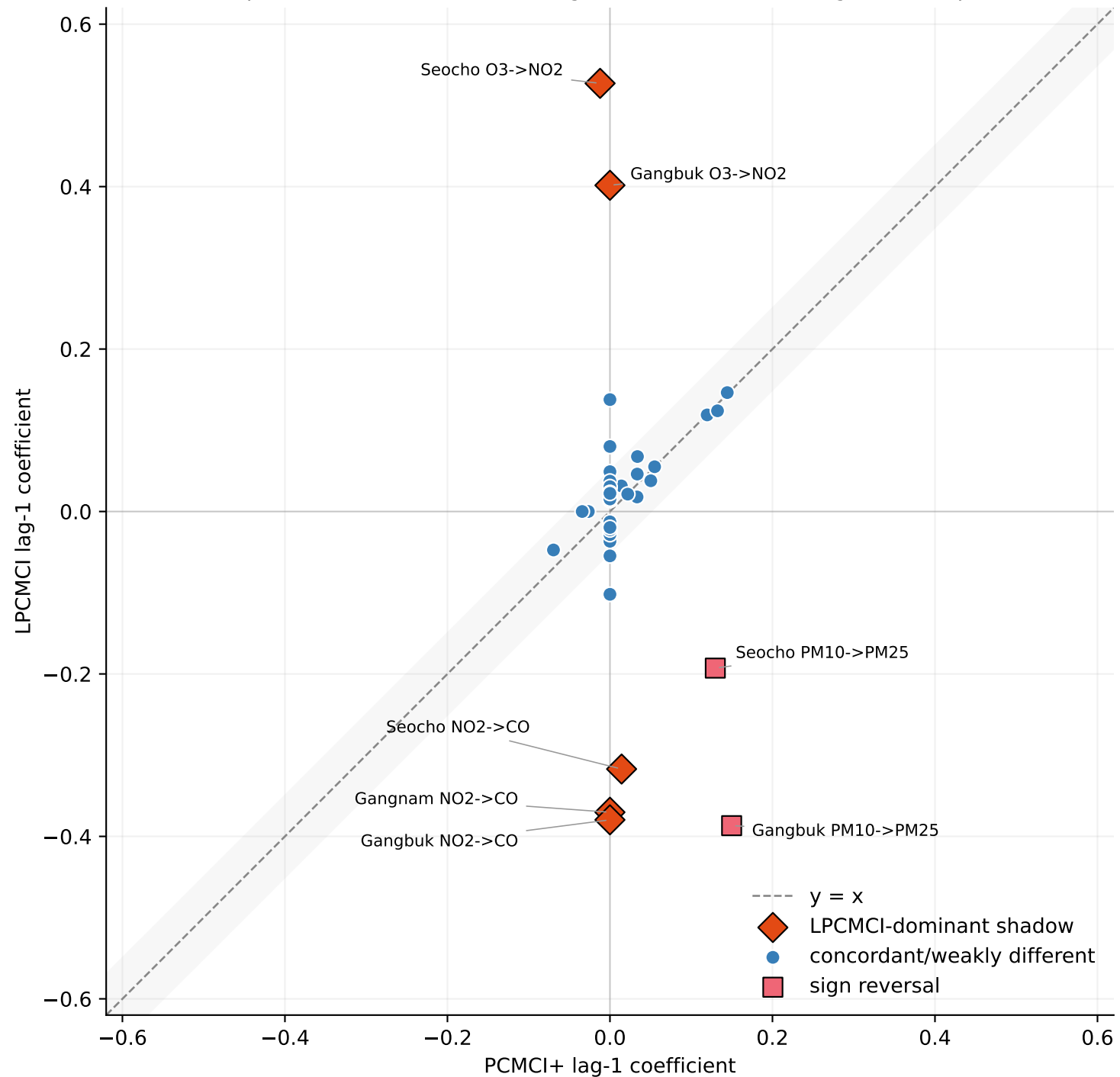
Lag-1 directed pollutant edges: PCMCi+ versus LPCMCI Three representative stations; off-diagonal values indicate algorithm dependence
