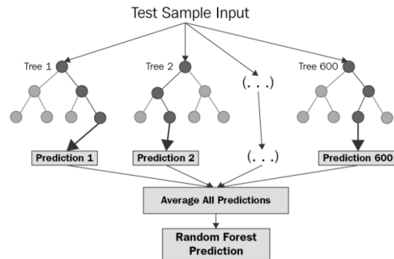
Figure 1: Sample Random Forest Regression Model
