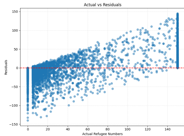
Figure 5: Actual vs. Residuals Plot
