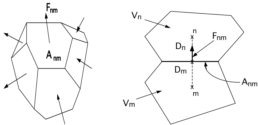
Figure 3.5-1 Space discretization and geometric data for the integral finite difference method (Pruess et al., 1999)
