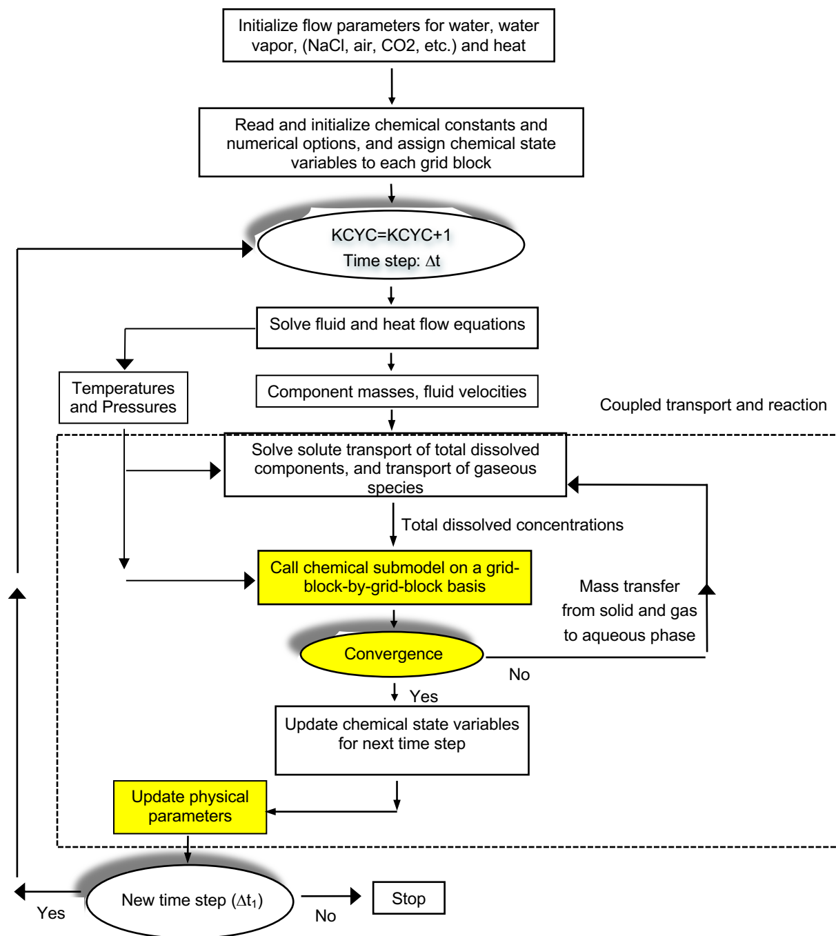
Figure 3 Flow chart of the TOUGHREACT program
