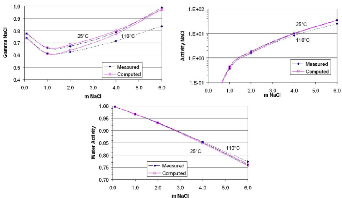
Figure H.1—4 Comparison of measured (Colin et al. 1985) and computed activities for NaCl solutions. Note that the \text{NaCl}_{(\text{aq})} species is excluded from the simulation for consistency with the activity coefficient model.
