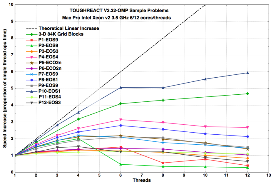
Figure 1. Increase in speed for sample problems as a function of the number of threads (ratio of cpu time for 1 thread to cpu time for multiple threads). Tests were performed on a Mac Pro workstation (late 2013 model) with an Intel Xeon 6-core (12-thread) 3.5 GHz E5 processor using MacOS 10.12.5 (Sierra). Both platforms show about the same performance until the number of threads exceeds the physical cores on the Mac Pro (6), at which point the Linux cluster with more physical cores and threads shows better parallel performance.
