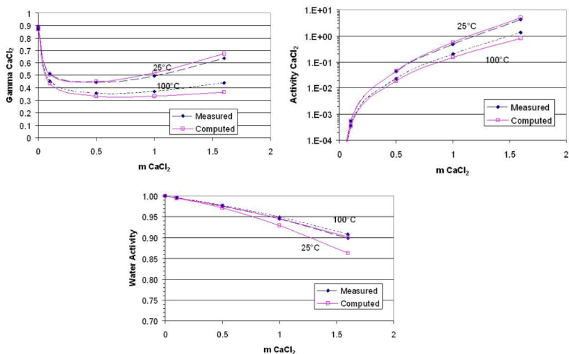
Figure H.1—5 Comparison of measured (Ananthaswamy and Atkinson, 1985) and computed activities for \text{CaCl}_2 solutions. Note that the \text{CaCl}_{2(\text{aq})} and \text{CaCl}^+ species are excluded from the simulation for consistency with the activity coefficient model.
