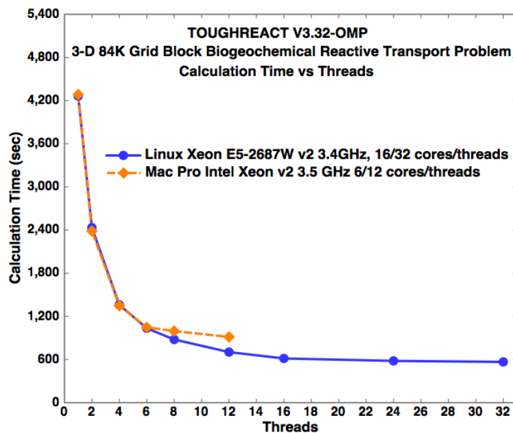
Figure 2. Calculation times (seconds) for a 3-D 84,000 grid block biogeochemical reactive transport problem on Linux Xeon and Mac Pro workstations using TOUGHREACT V3.32-OMP. Results for the current version are roughly equivalent.
