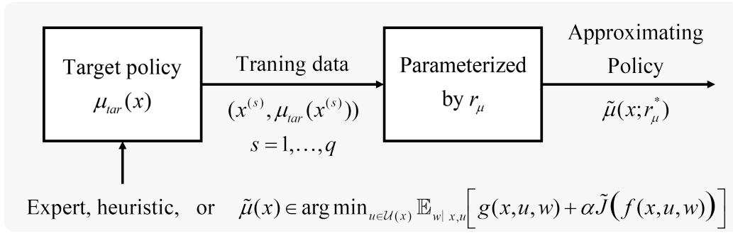
Figure 1.11: Policy-space approximation by fitting target actions supplied by an expert, heuristic, classical controller, or value-based improvement procedure.
